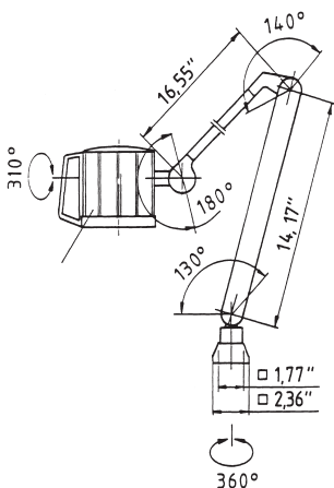
HG-55 32" Arm
