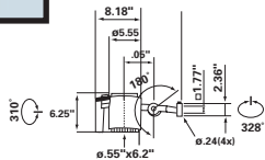
HSW-75 32" Arm
