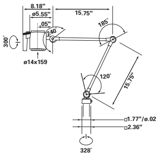
HSW front ring bayonet allows for quick and easy lamp replacement
