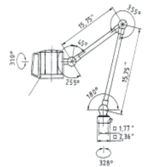
HGW ARTICULATING ARM
