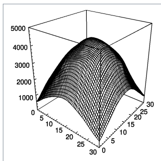
illuminancefield 35 cm
