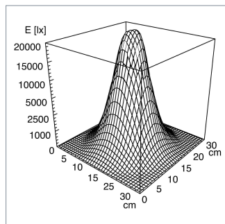
illuminancefield 6 cm
