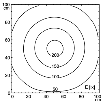
measuring conditions: d=50cm
