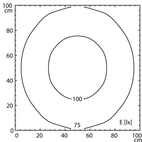
light distribution
