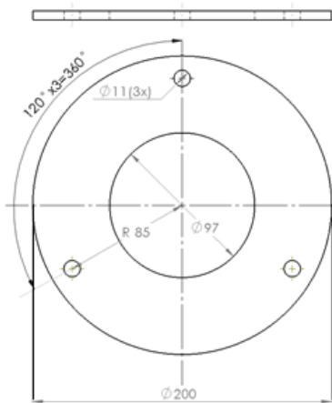
Mounting Base Template (Not to scale)
